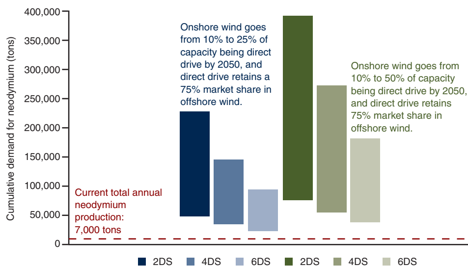
FIGURE 2.2 Ranges for Cumulative Neodymium Demand for Global Wind Turbine Production through 2050
