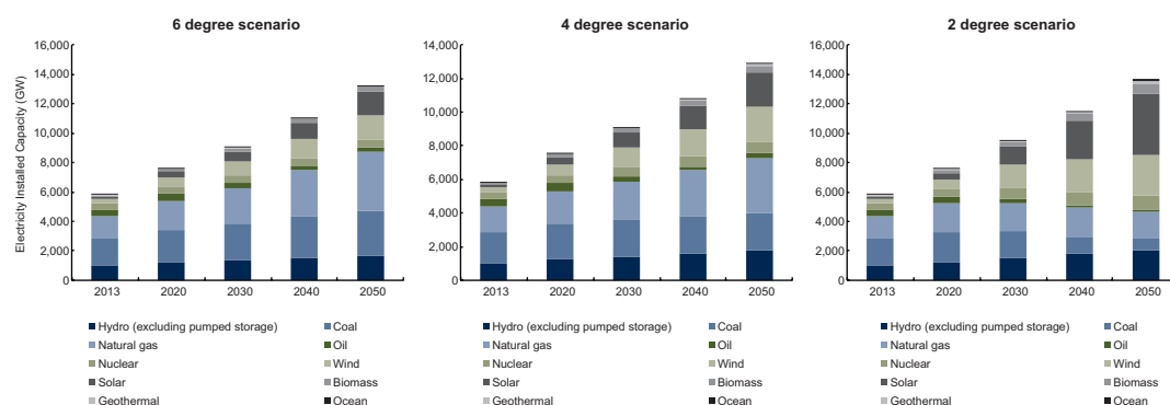
FIGURE 1.1 IEA Technology Scenarios for Electricity Installed Capacity
